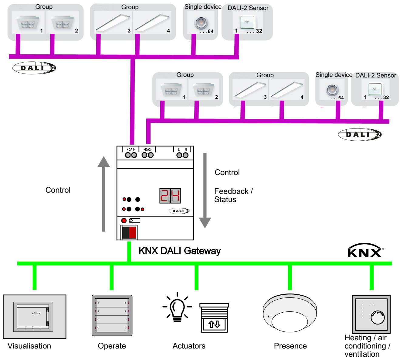
Figure 12: Principle overview of a KNX-DALI system integration with DALI sensors (example)
