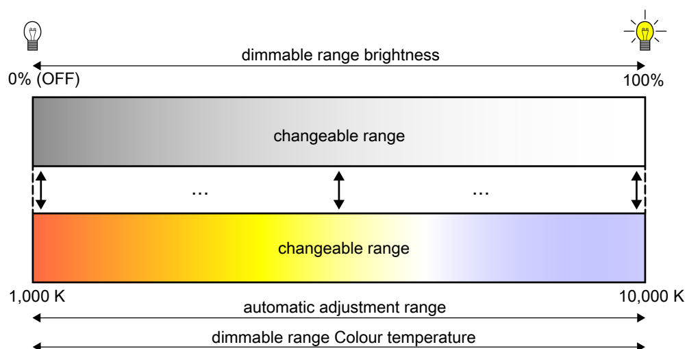
Figure 28: Automatic adjustment of the colour temperature to the set brightness Example in the maximum brightness and colour temperature range
