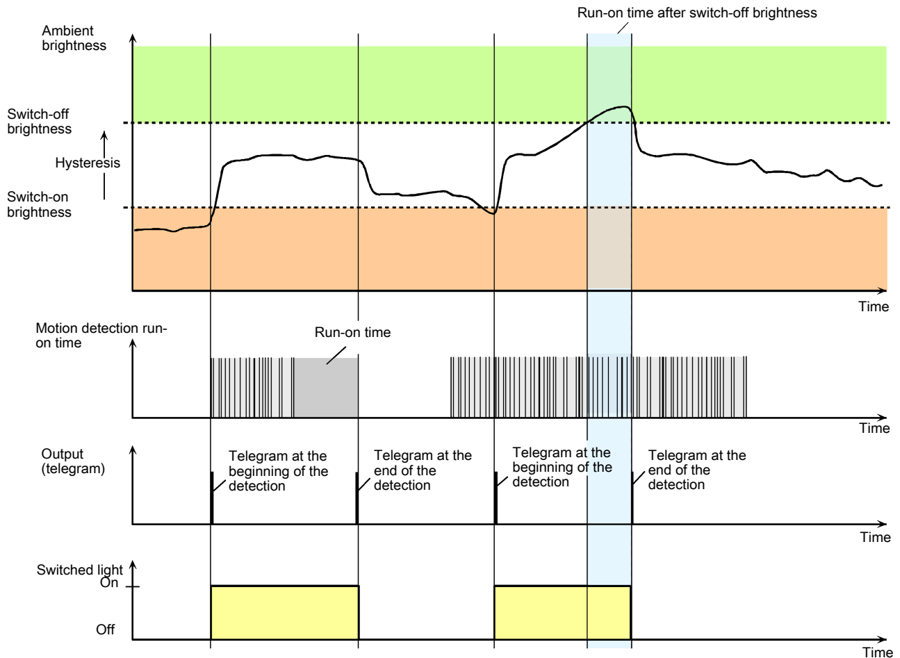
Figure 66: Brightness-dependent presence detection
