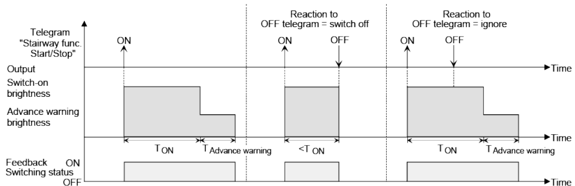
Figure 54: Switch-off behaviour of the staircase function without soft functions
