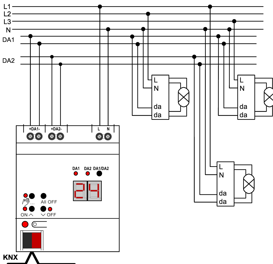
Figure 4: DALI gateway connection example, 2fold
