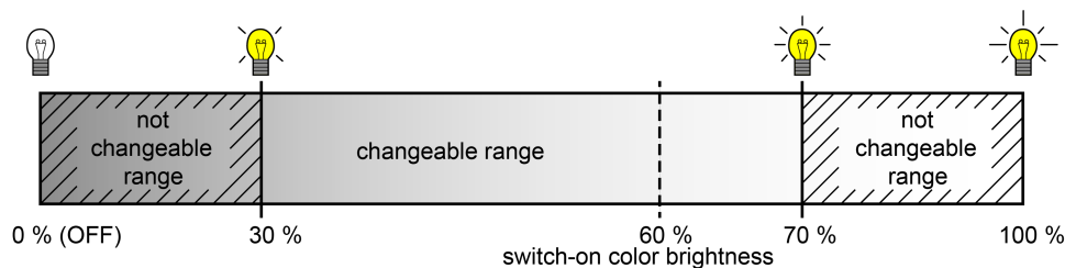
Figure 20: Example of a brightness range with switch-on brightness
