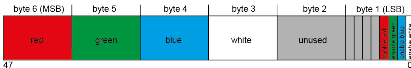
Figure 36: KNX data type "RGBW combined" (DPT 251.600)
