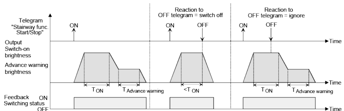
Figure 55: Switch-off behaviour of the staircase function with soft functions (as an example with minimum brightness = 0 %)
