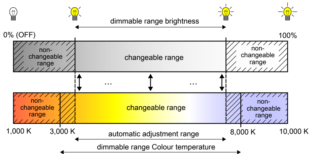
Figure 29: Automatic adjustment of the colour temperature to the set brightness Example with limited brightness and colour temperature range
