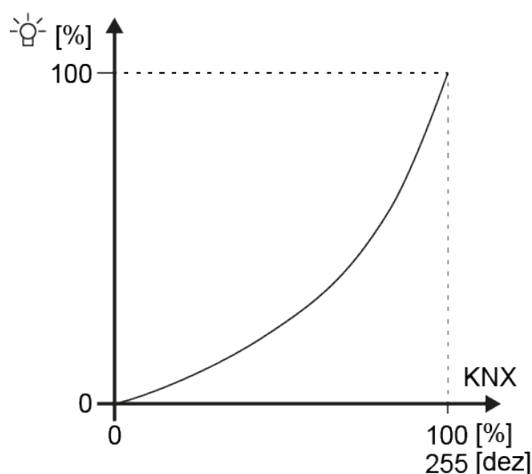
Figure 25: Combined dimming characteristic curve at the output of an operating device (relative luminous flux [%] depending on the 8-bit KNX data value [0...255])
