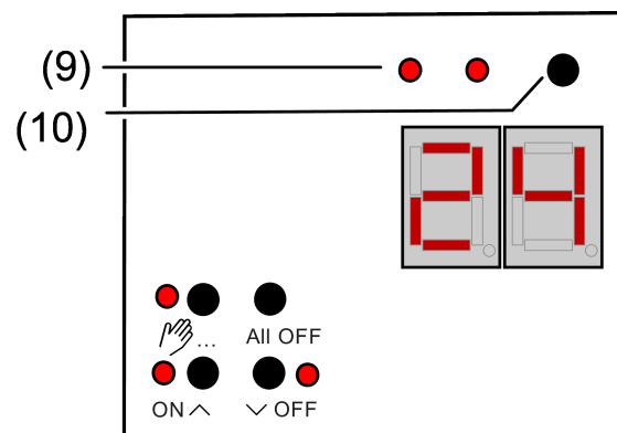
Figure 14: DALI gateway control panel, 2-gang
