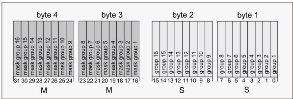
Figure 16: Structure of the objects of the collective feedback, using the example of the object for Groups 1-16
