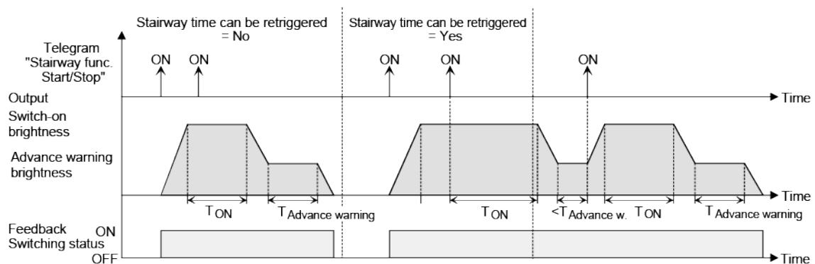
Figure 53: Switch-on behaviour of the staircase function with soft functions (as an example with minimum brightness = 0 %)
