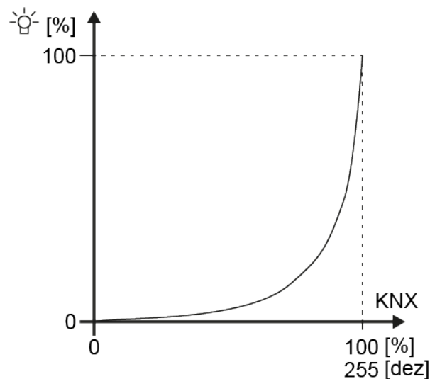
Figure 24: Logarithmic dimming characteristic curve at the output of an operating device (relative luminous flux [%] depending on the 8-bit KNX data value [0...255])
