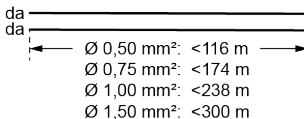
Figure 2: DALI cable length
