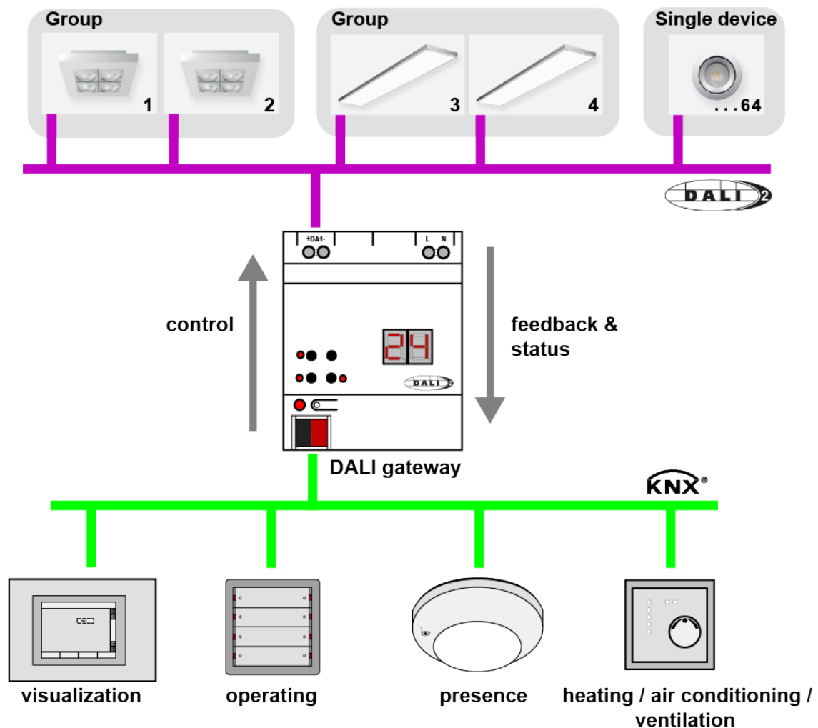
Figure 5: Principle overview of a KNX-DALI system integration
