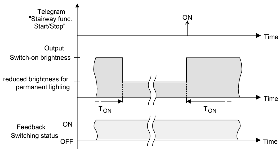
Figure 58: The continuous lighting of the staircase function without soft functions
