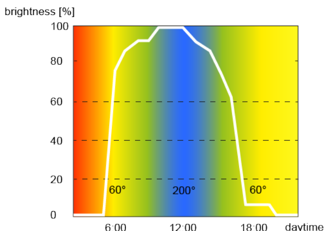
Figure 47: Exemplary daytime colour sequence with colour and brightness adjustment
