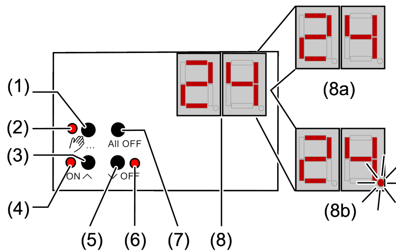
Figure 13: DALI gateway control panel, 1-gang
