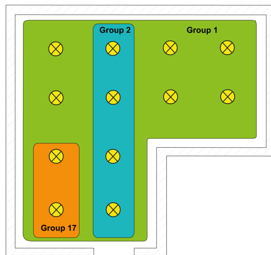
Figure 11: Example of multiple assignment of operating devices - Here: Group 1 overlaps with Group 2 and Group 17
