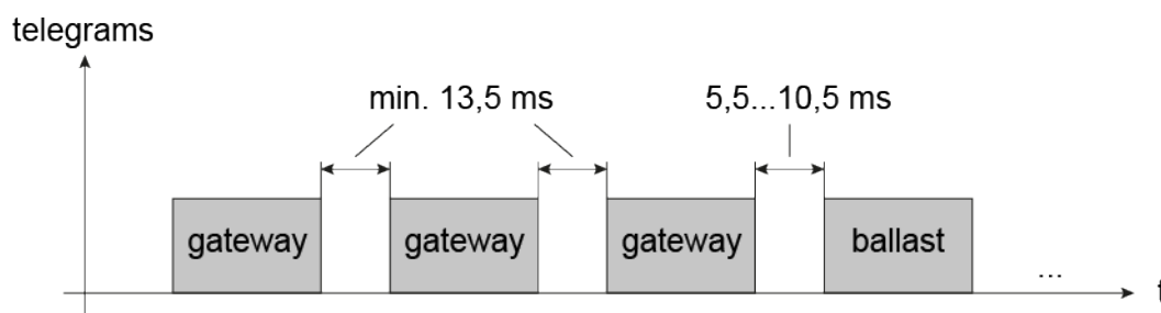
Figure 15: Pause times between DALI commands
