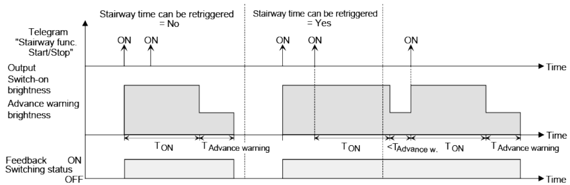
Figure 52: Switch-on behaviour of the staircase function without soft functions
