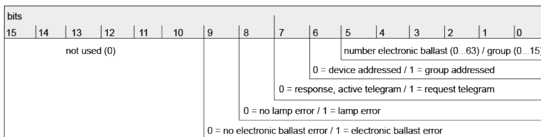
Figure 18: Telegram structure, 2-byte error status
