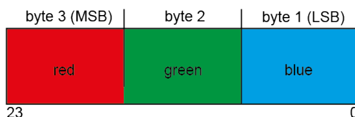
Figure 35: KNX data type "RGB combined" (DPT 232.600)
