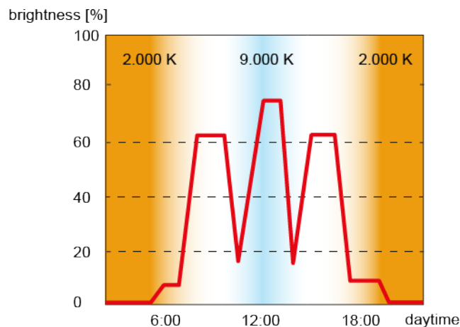
Figure 32: Exemplary daytime colour temperature sequence "Intensive learning"
