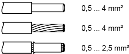
Figure 3: Clampable cable cross-sections
