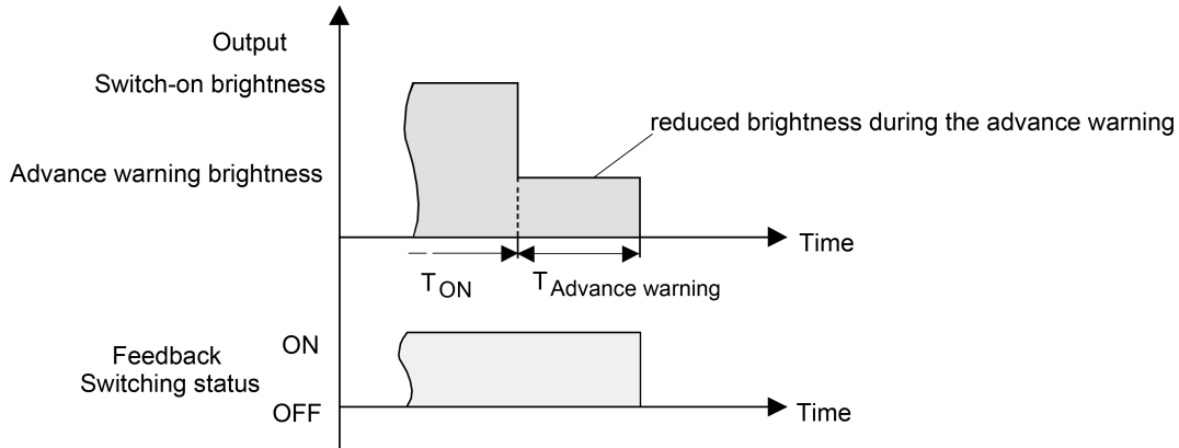
Figure 56: The pre-warning function of the staircase function without soft OFF function
