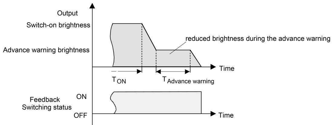
Figure 57: The pre-warning function of the staircase function with soft OFF function (as an example with minimum brightness = 0%)
