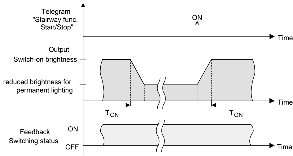
Figure 59: The continuous lighting of the staircase function with soft OFF functions
