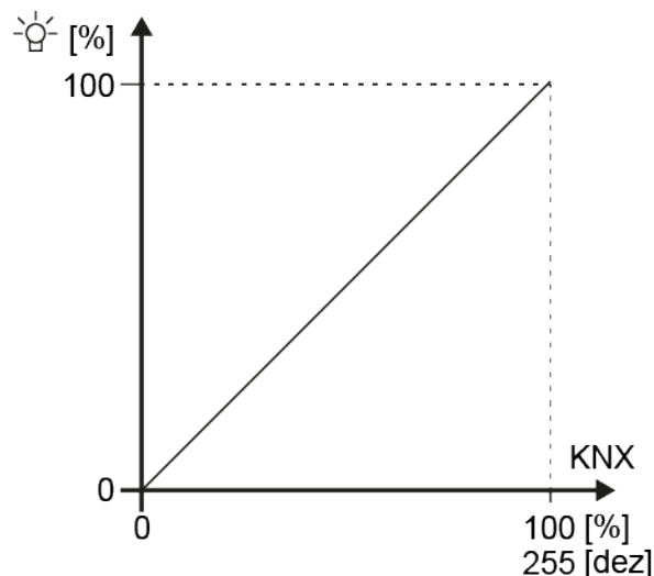
Figure 23: Linear dimming characteristic curve at the output of an operating device (relative luminous flux [%] depending on the 8-bit KNX data value [0...255])
