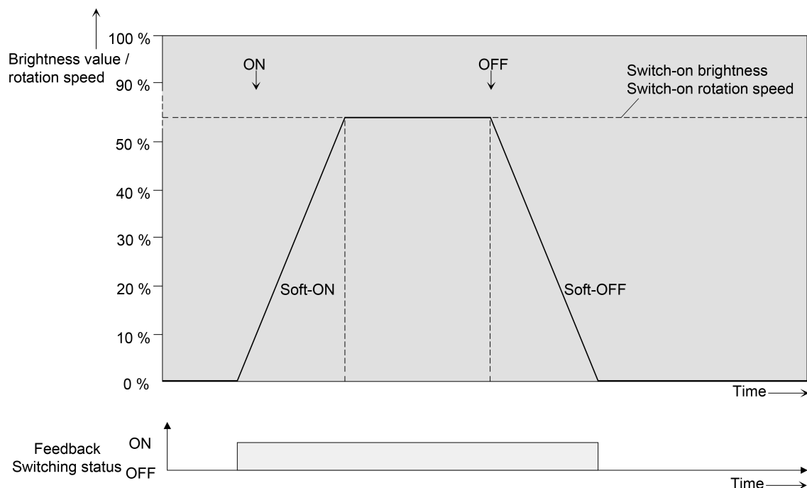
Figure 50: Dimming behaviour of the soft ON/OFF functions as an example with minimum brightness > 0%
