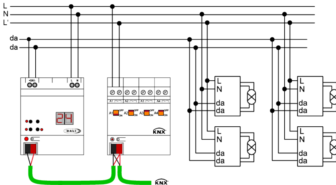
Figure 19: Example of a connection diagram for standby switch-off by a KNX switching actuator
