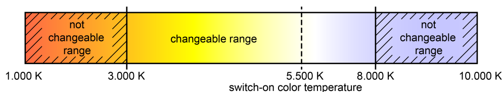
Figure 26: Example of a configured colour temperature range with switch-on colour temperature
