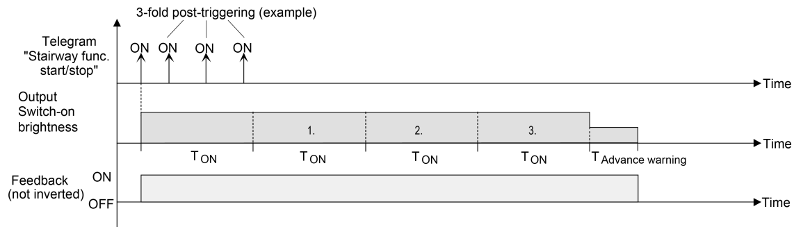
Figure 60: Time extension of the staircase function
