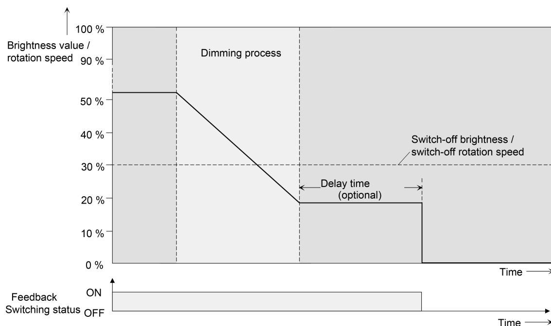
Figure 51: Dimming and switching behaviour of the automatic switch-off function
